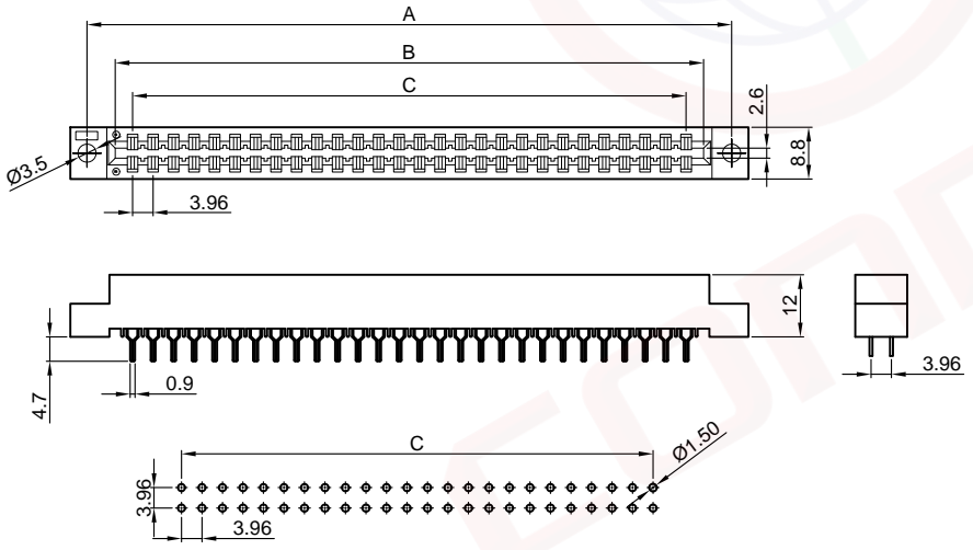
Recommend PCB layout
