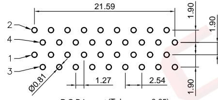
P.C.B Layout (Tolerance:±0.05) For Positions 20,40,60,68,80,100
