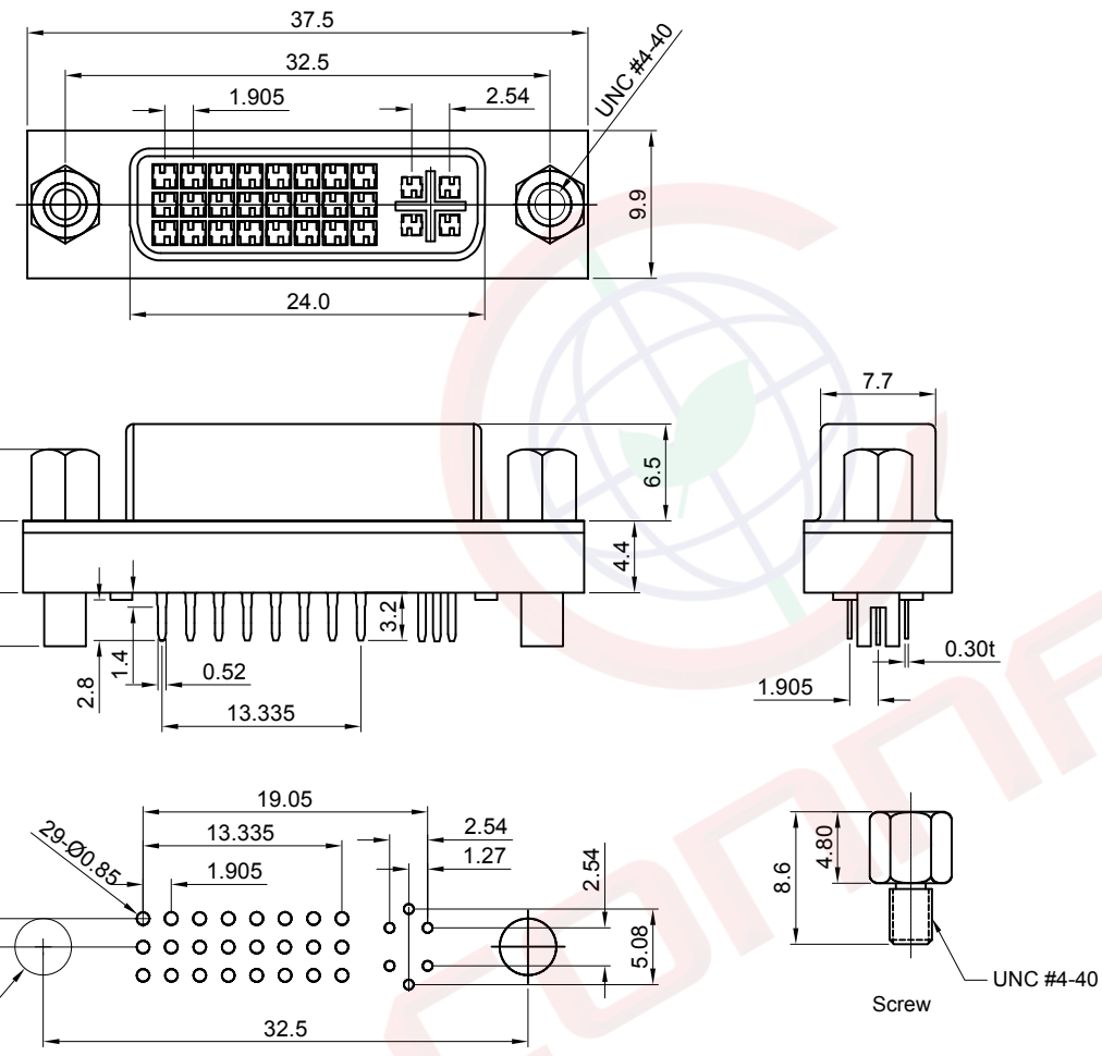
Recommend PCB Layout (Tolerance:±0.05)
